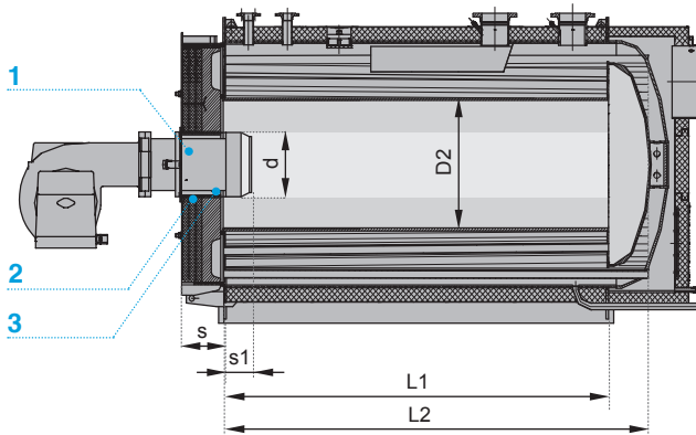
Burner installation
